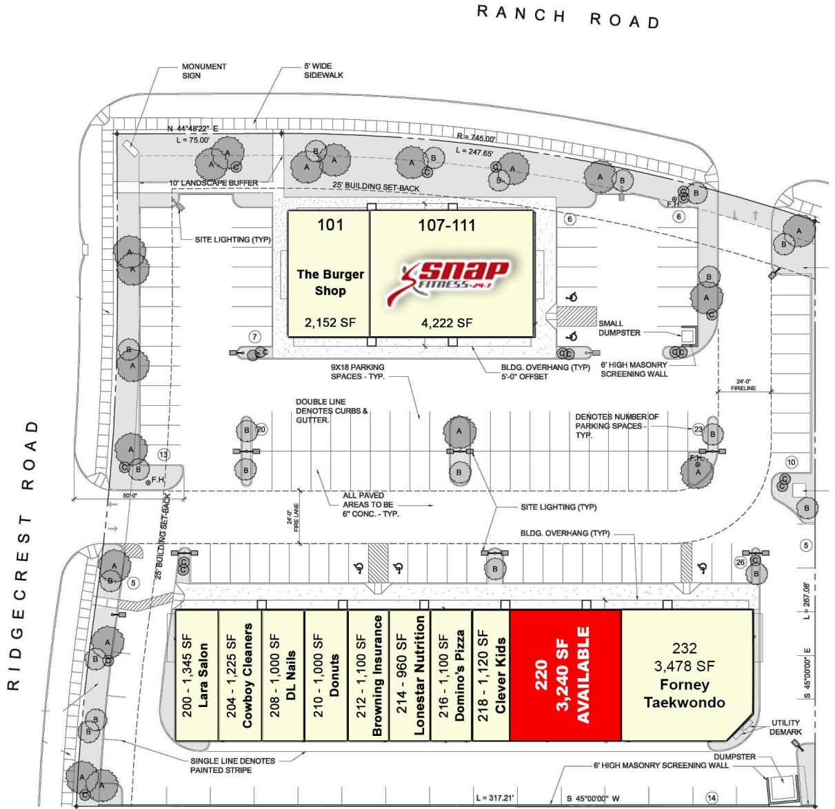
1 Site Plan 1" = 20'-0"
